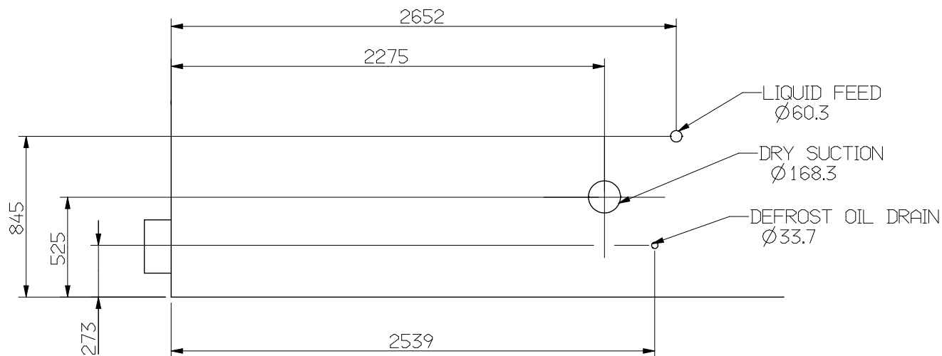
TOP VIEW LVS CONNECTION
