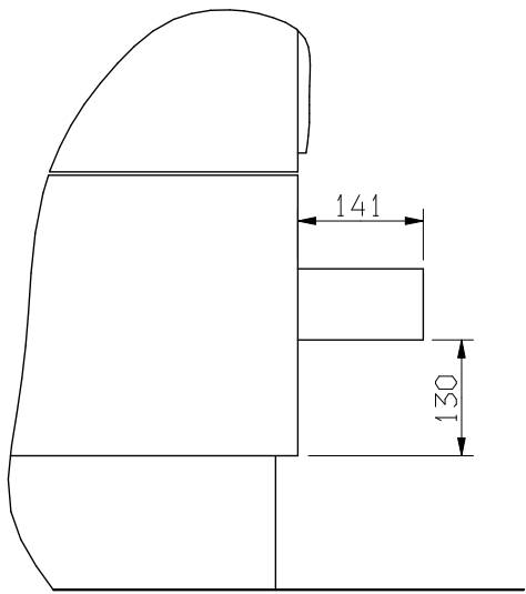
DETAIL A SCALE 3:20
